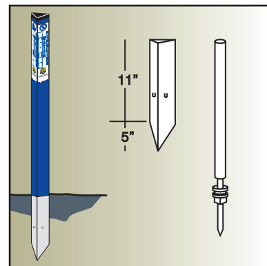
Side - TriView Front - TriView Side - TriView Side - 3-Rail Front - 3-Rail VIEWS OF THE RHINO TRIVIEW COMPARED TO VIEWS OF A RHINO 3-RAIL FIBERGLASS POST
